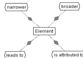
Figure 1. Ontology Scheme
