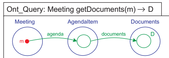
Figure 3: Query.
